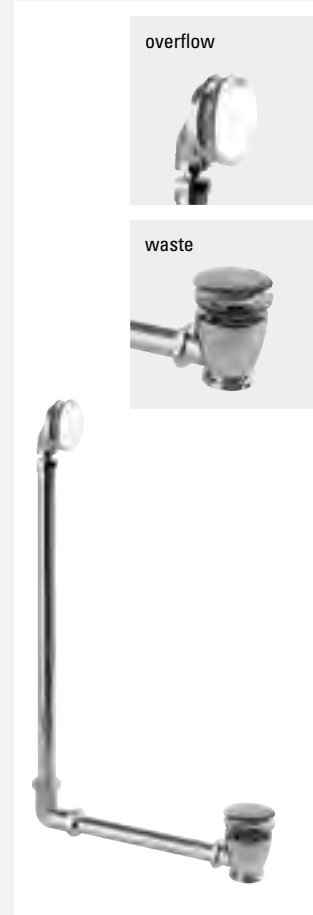
Exposed bath overflow, click-clack waste D: 318, W: 75, H: 565 Code: CW6 Price: £169
