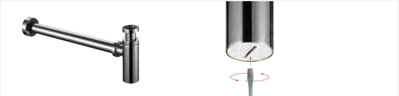
Flat bottom basin bottle trap D: 362, W: 67, H: 180 Pipe length can be cut to size on site Code: W13 Price: £89
