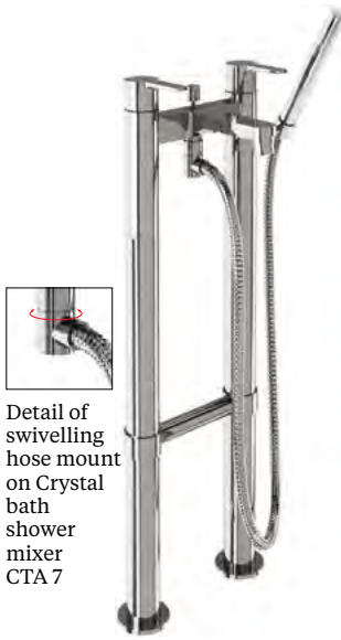
Bath shower mixer on stand pipes Floor standing 17.5cm x 30.2cm x 89.5cm Bath filler CTA7 Stand pipes W7
