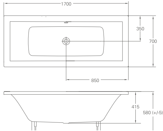
Enviro Baths & Panels Double ended - Square internal
