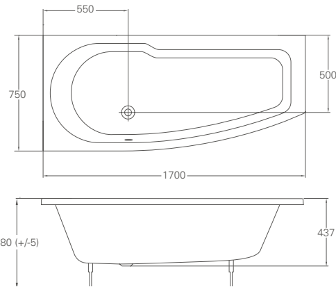
EcoCurve showering bath, page 122
