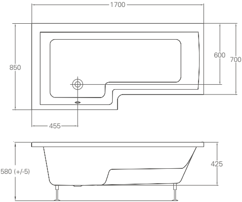
EcoSquare showering bath, page 123
